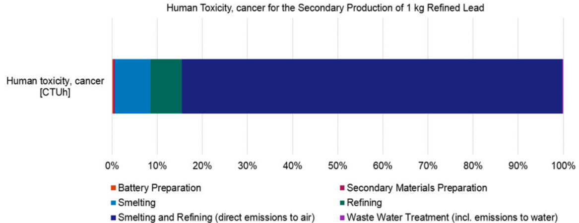
Figure C-3: Human toxicity (cancerous) for the secondary production of 1 kg refined lead
