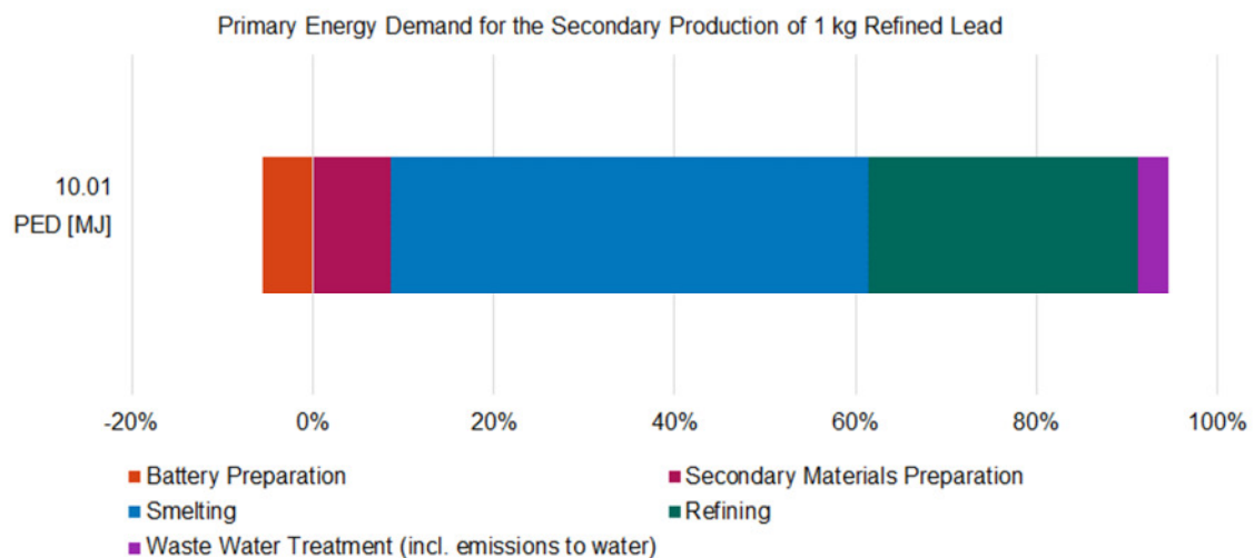
Figure 4-1: PED for the secondary production of 1 kg refined lead
