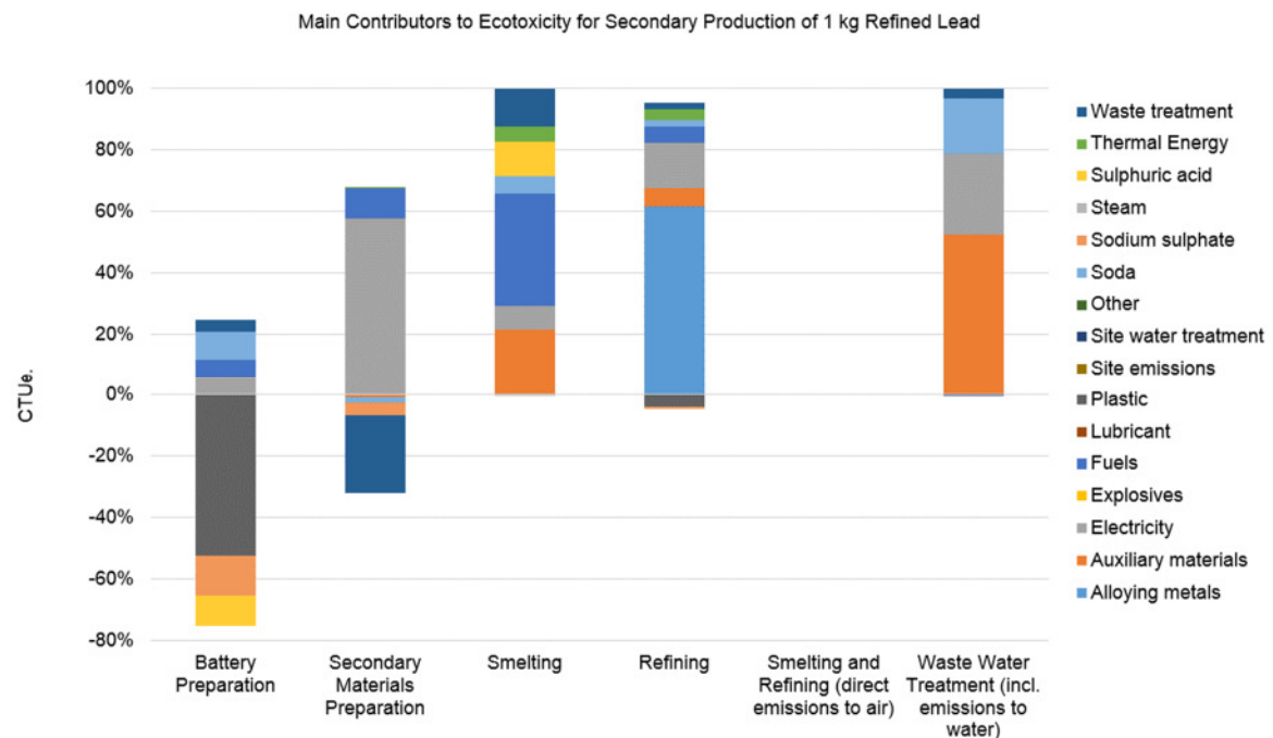
Figure C-2: Main contributors to the Ecotoxicity for the secondary production of 1 kg refined lead
