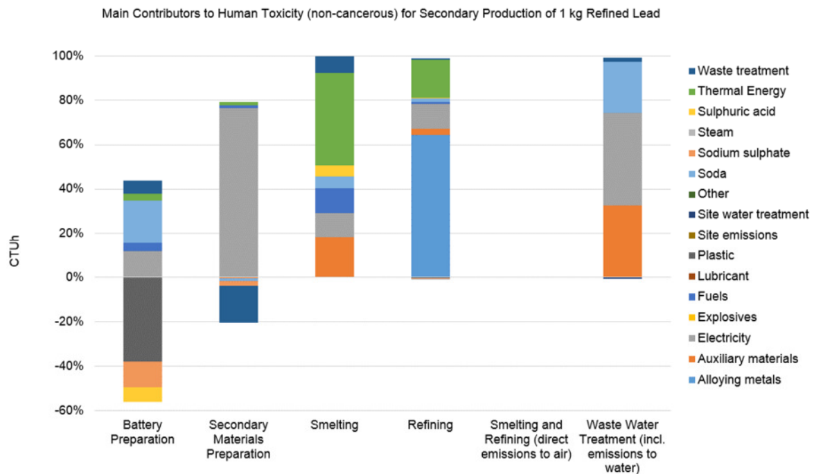
Figure C-6: Main contributors to the Human toxicity (non-cancerous) for the secondary production of 1 kg refined lead
