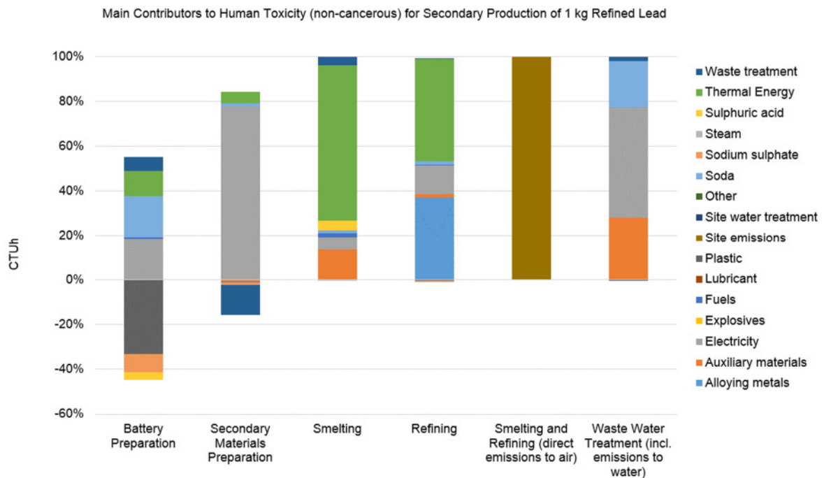
Figure C-4: Main contributors to the Human toxicity (cancerous) for the secondary production of 1 kg refined lead
