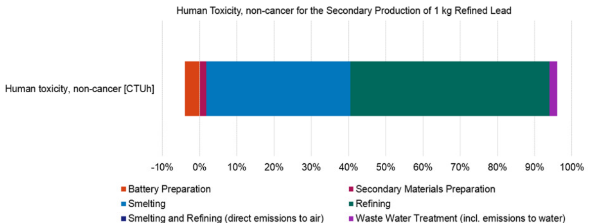
Figure C-5: Human toxicity (non-cancerous) for the secondary production of 1 kg refined lead
