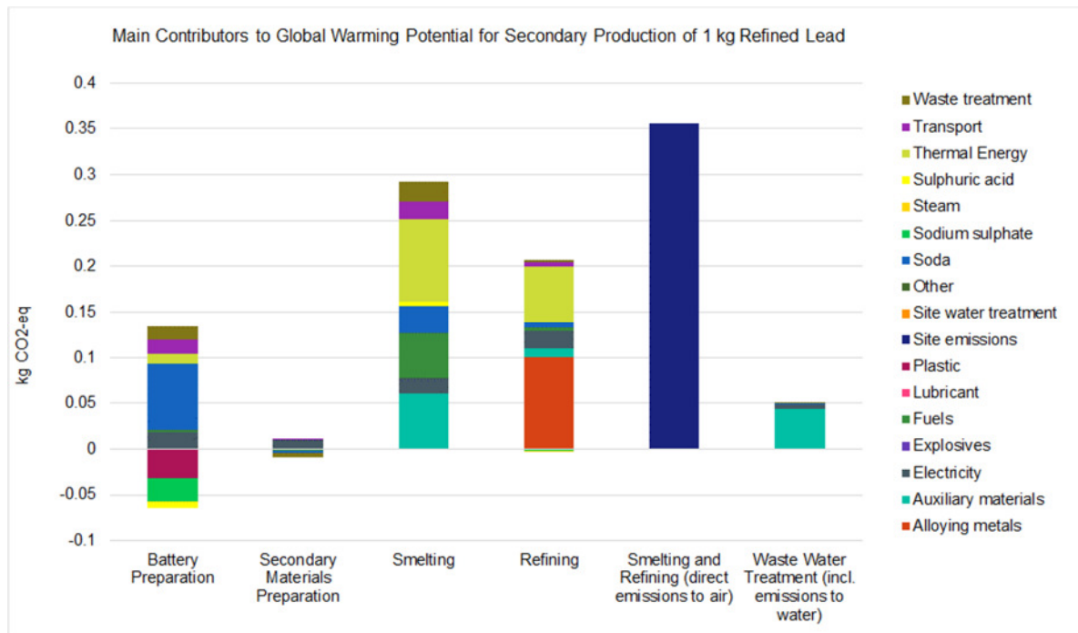
Figure 4-4: Main contributors to the GWP for the secondary production of 1 kg refined lead
