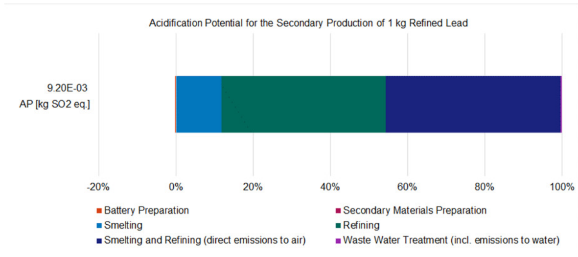
Figure 4-5: AP for the secondary production of 1 kg refined lead
