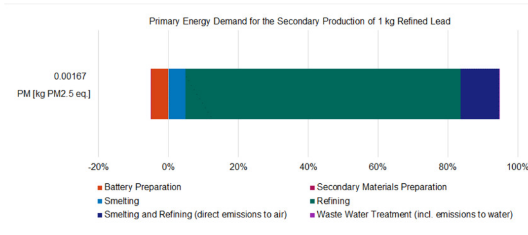
Figure C-7: Relative particulate matter results, by product stage, secondary route
