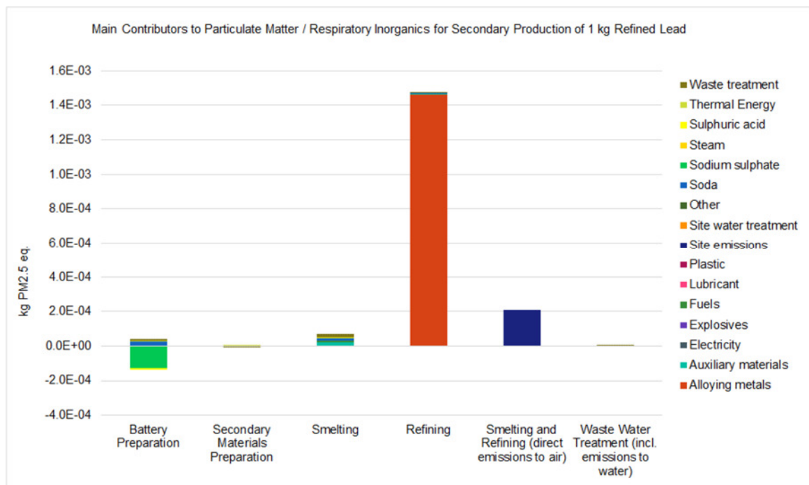
Figure C-8: Main contributors to the particulate matter for the secondary production of 1 kg refined lead
