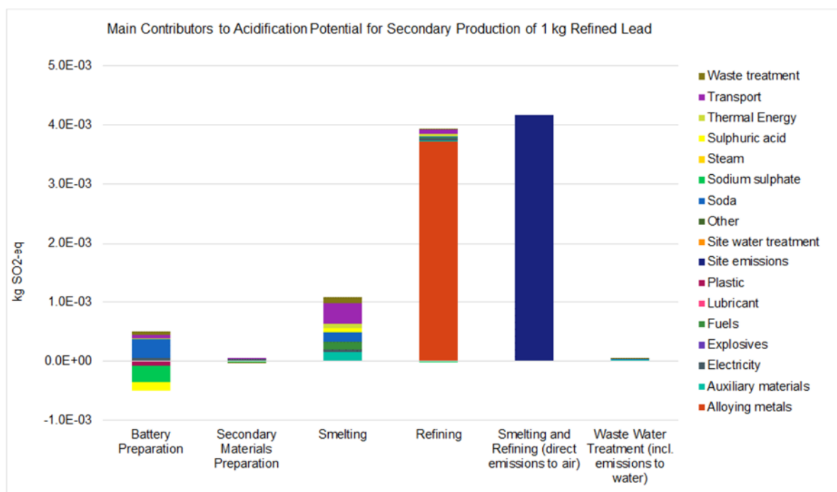
Figure 4-6: Main contributors to the AP for the secondary production of 1 kg refined lead
