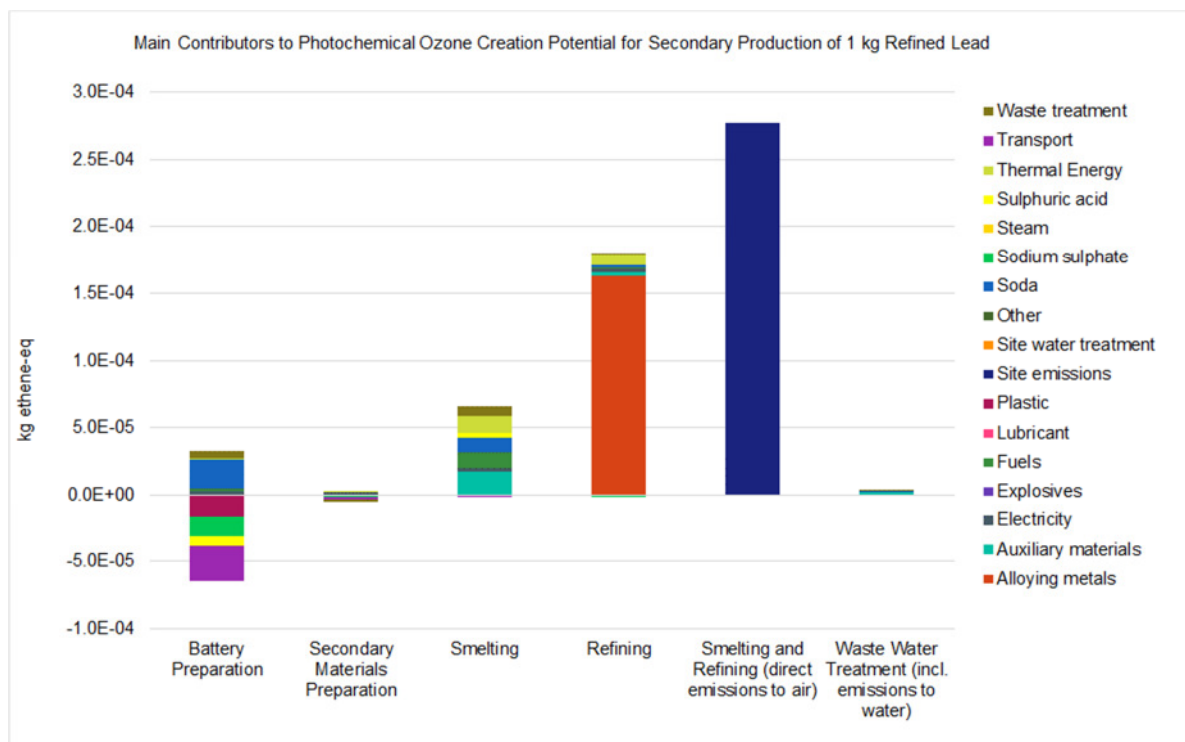
Figure 4-10: Main contributors to the POCP for the secondary production of 1 kg refined lead
