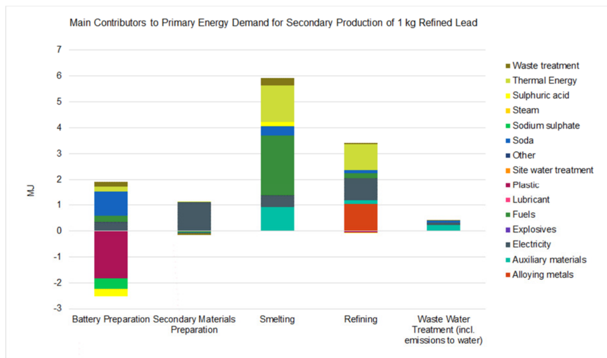
Figure 4-2: Main contributors to the PED for the secondary production of 1 kg refined lead
