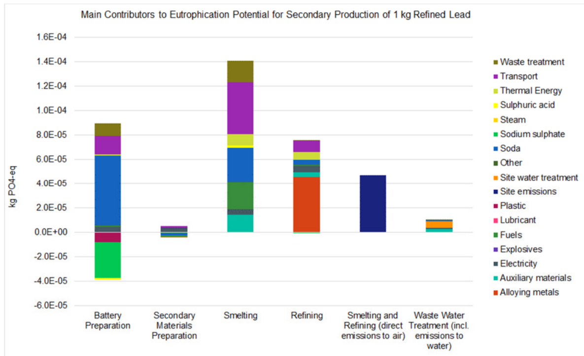
Figure 4-8: Main contributors to the EP for the secondary production of 1 kg refined lead
