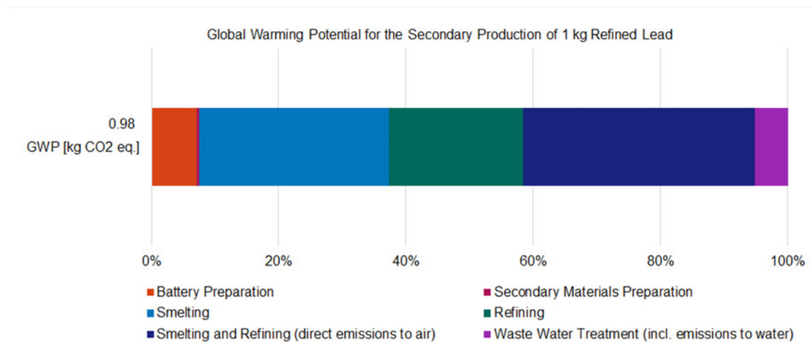
Figure 4-3: GWP for the secondary production of 1 kg refined lead
